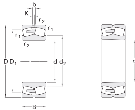
Cylindrical bore
