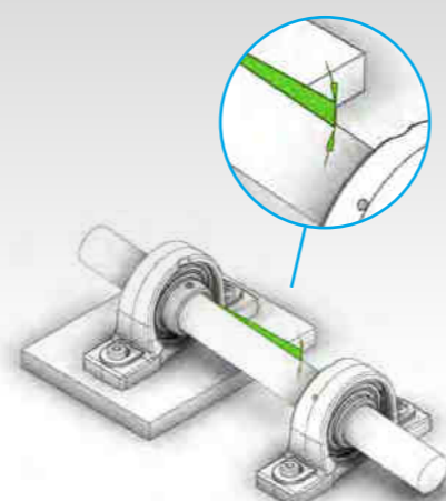
Bearing units can cope with a high degree of mounting errors
